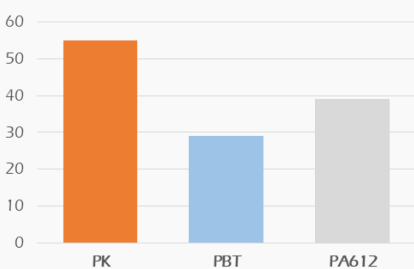
Graph.5 Bend Recovery %
